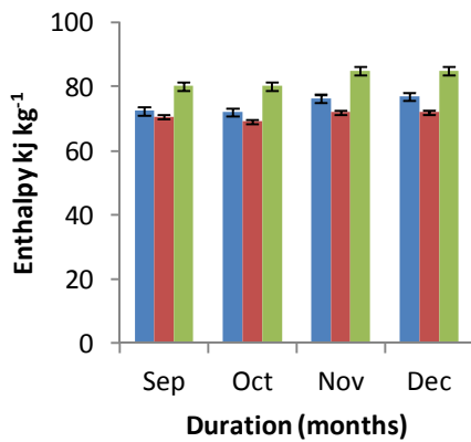
Fig. 6 Enthalpy in storage structures
