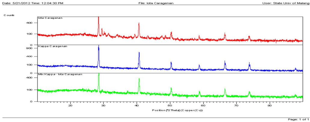
Figure 3 the test results are mixed carrageenan Eucheuma spinosum and Eucheuma cottonii using X-ray Diffraction
