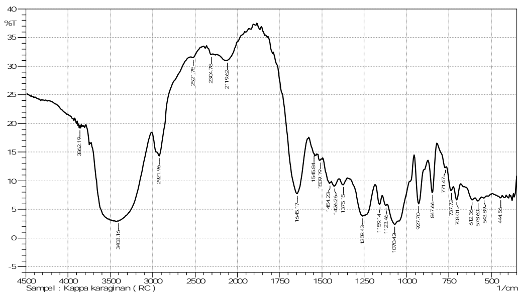
Figure 1 Characteristic functional groups Carrageenan of Eucheuma cottonii species using FTIR
