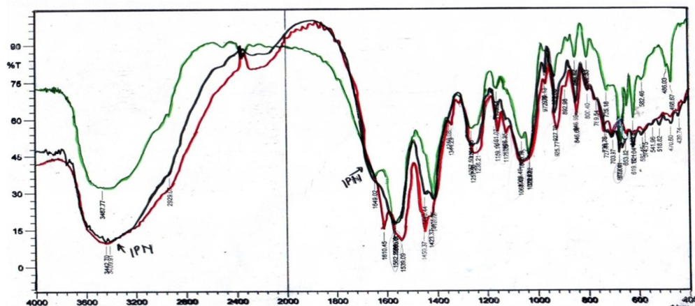
Figure 4 kappa, iota and mixture kappa-iota carrageenan functional group using FTIR
