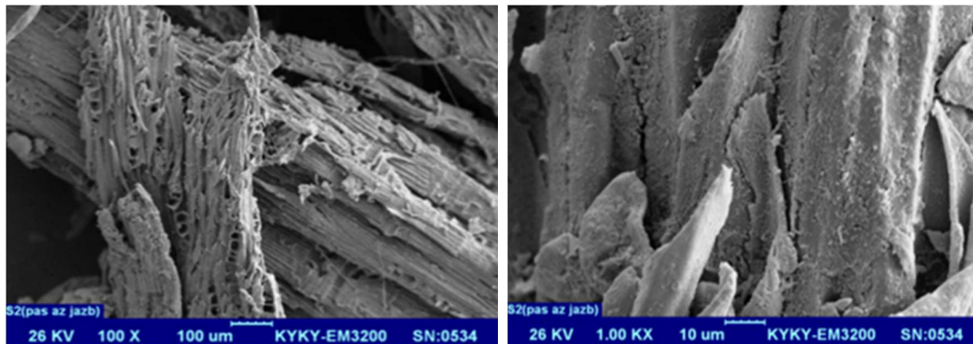
Figure 10. SEM images after adsorption of metal by myrtaceae sawdust with 100X and 1KX magnifications
