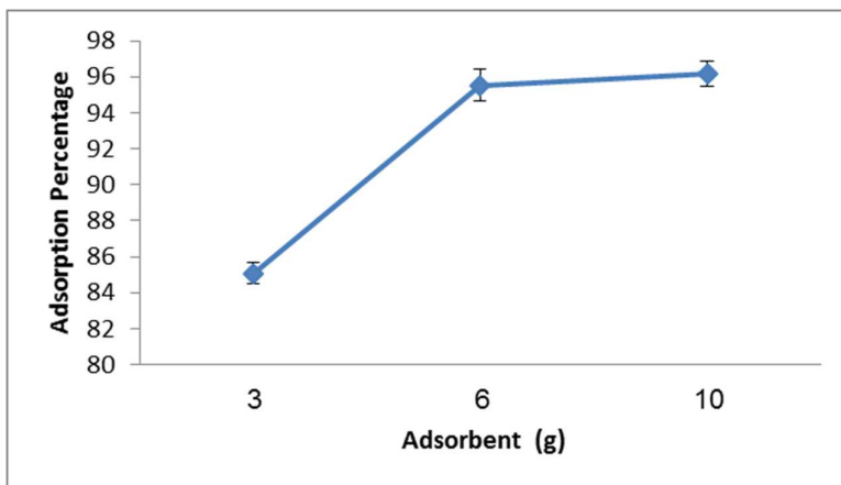
Figure 2. Effect of different adsorbent quantity on adsorption percentage of lead (pH=7, Contact time=30 min, Initial concentration of lead=10 mg/L)
