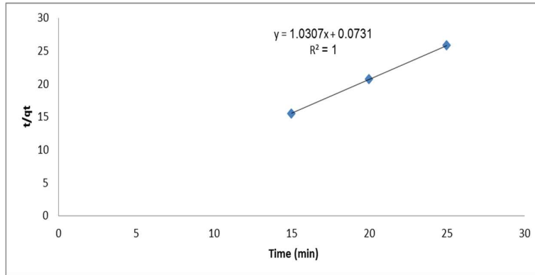
Figure 8. Second-degree adsorption kinetic model
