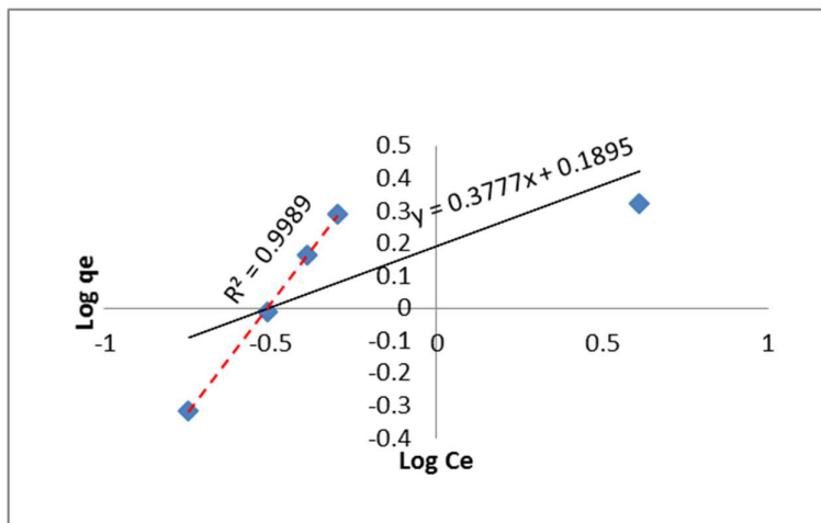
Figure 6. Freundlich isotherm model for lead adsorption
