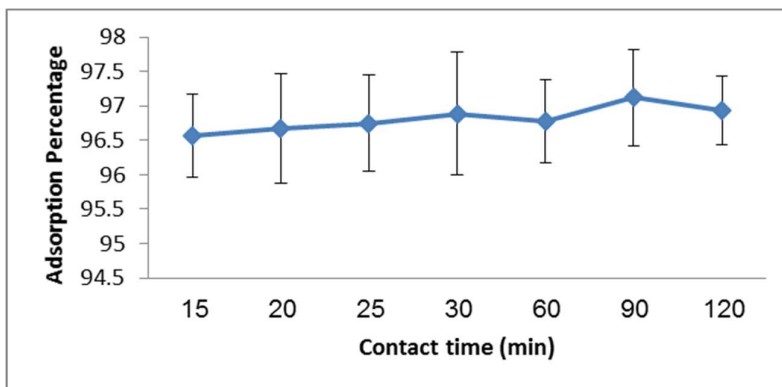
Figure 3. Effect of different contact times on the adsorption percentage of lead (pH=7, Adsorbent quantity = 10 g/L, Initial concentration of lead=10 mg/L)
