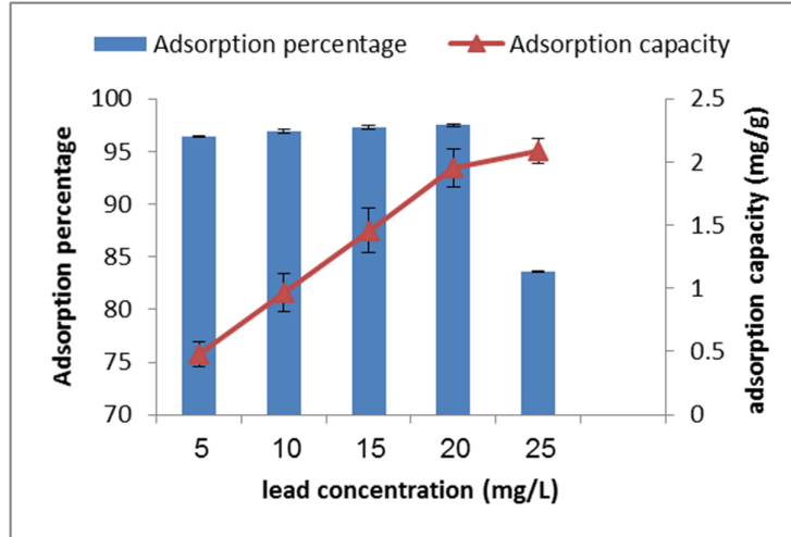
Figure 4. Effect of the quantity of different initial concentration on the capacity and percentage of lead (pH=7, Adsorbent quantity =10 g/L, Contact time=30 min)
