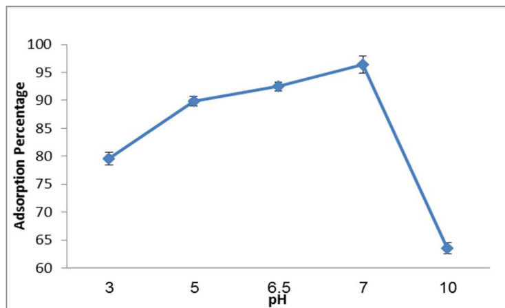
Figure 1. Effect of various pH on the adsorption percentage of lead (Adsorbent quantity =10 g/L, Contact time=30 min, Initial concentration of lead=10 mg/L)
